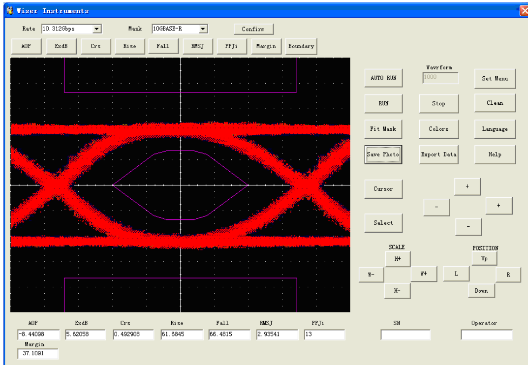
10 Gb/s Eye-diagram
